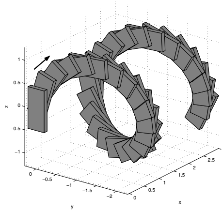
Fig. 6.8 Motion of a rigid body with constant spatial velocity of \mathbf{v}_o = [0.3 \ 0 \ 1]^T (m/s), \boldsymbol{\omega} = [1 \ 0 \ 0]^T (rad/s). State of every 0.3 second is displayed during the motion of 10 seconds. A trajectory of a rigid body with constant spatial velocity generally becomes a spiral.
