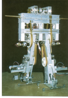
Gifu Univ. Kenkyaku 2 (1983)
