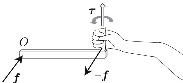
Fig. 6.30 The answer for the quiz of page 207: To keep the rod stationary, a person must apply the force -\mathbf{f} as well as the moment \tau . If the person who is gripping the handle is on a small boat, he/she will start moving in the direction of vector \mathbf{f} .
