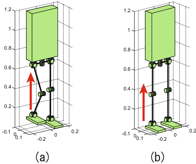
Fig. 2.32 Non-singular posture and singular posture
