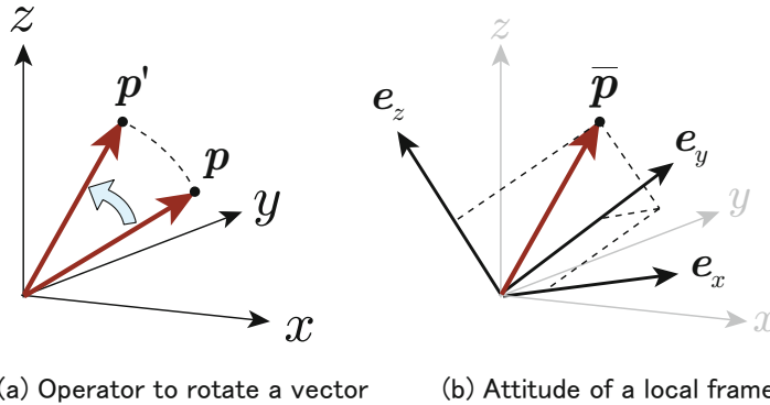
Fig. 2.6 Two ways to interpret rotation matrices
