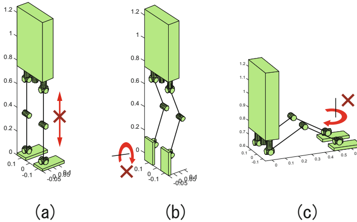
Fig. 2.33 Singular posture examples. In these postures there exist directions in which the end point cannot move (shown with arrows). In these cases the Jacobian inverse cannot be solved.
