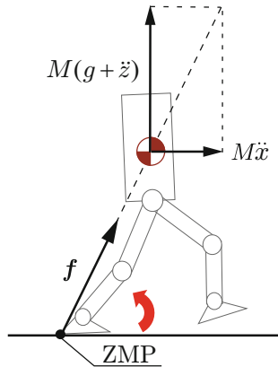
Fig. 3.29 The robot begins to rotate about the heel since the ZMP exists at the heel due to the highly accelerated center of mass. Since the acceleration in the vertical direction is generated, the ZMP remains in the support polygon.
