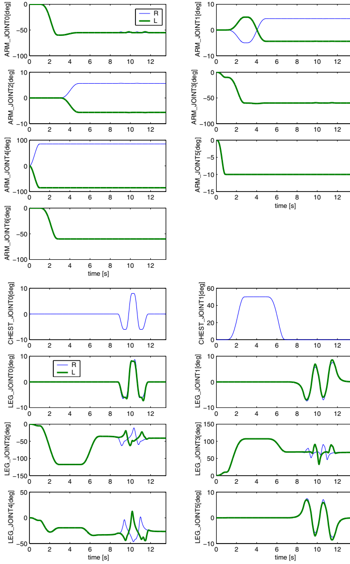
Fig. 5.2 Time Graph of the major joints on the HRP-2. First 7[s] are lifting the box, 7 to 13[s] is the walking motion.
