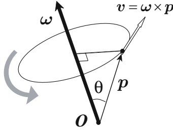
Fig. 2.8 Definition of Cross Product. \mathbf{v} = \boldsymbol{\omega} \times \mathbf{p} represents the velocity of the a point on the circle. It is at right angles to both \boldsymbol{\omega} and \mathbf{p} .
