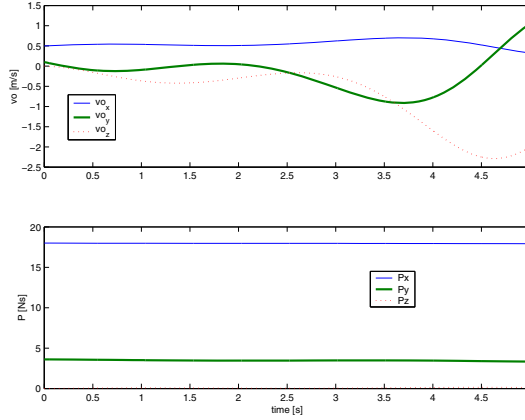
Fig. 6.10 The spatial velocity v_o and the linear momentum \mathcal{P} of the simulation of Fig. 6.9. v_o changes in time while \mathcal{P} keeps constant corresponding the linear constant speed of the center of mass.
