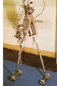
Tokyo Inst.Tech. BIPMAN2 (1982)
