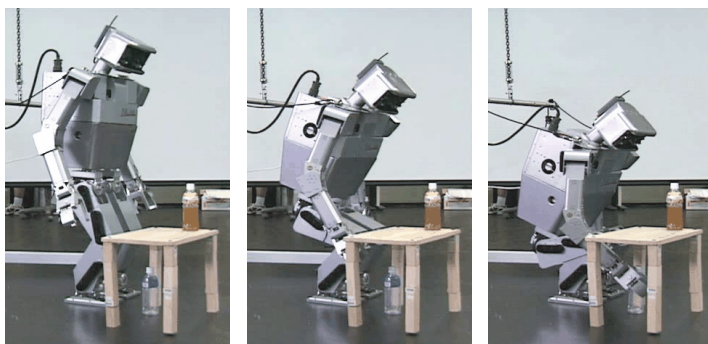
Fig. 5.11 Conversion Using an Auto-Balancer (Photograph Courtesy of JSK Lab. University of Tokyo)
