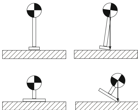
Fig. 5.19 Relation Between Static Stability and Hight of Center of Mass and Supporting Polygon Size
