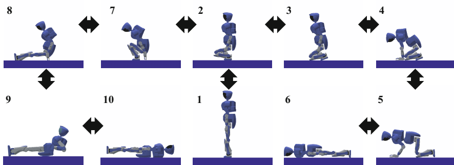
Fig. 5.23 State Chart for Stand Up Motion
