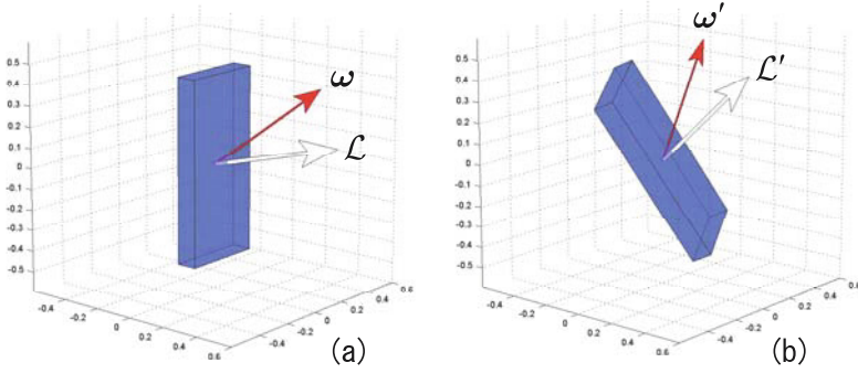
Fig. 3.19 (a) Angular Velocity Vector \omega and Angular Momentum Vector \mathcal{L} of a Rigid Body (Reference Posture) (b) Rotation of Rigid Body (Relative position of both vectors \omega' and \mathcal{L}' with respect to the rigid body do not change.)
